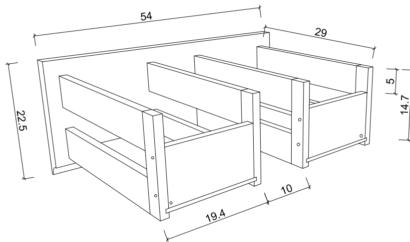
DETAIL DRAWER
