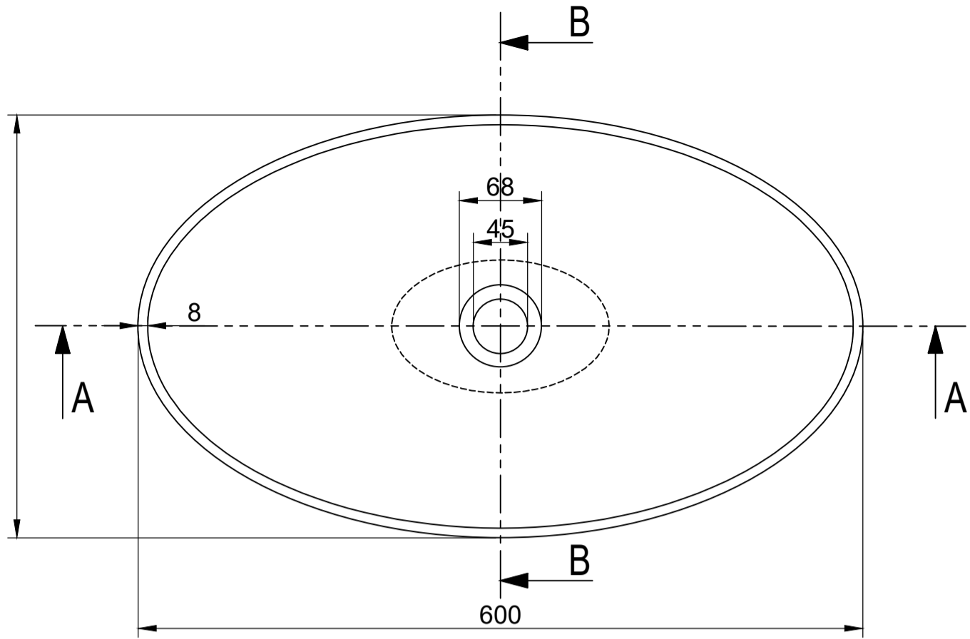
TOP VIEW
