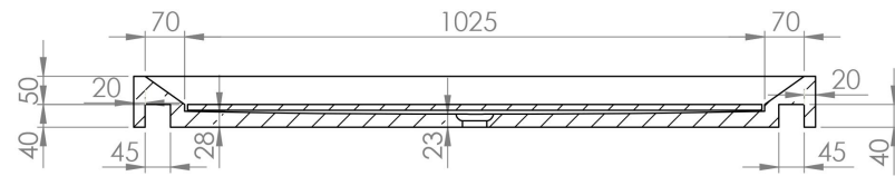
SECTION B-B
