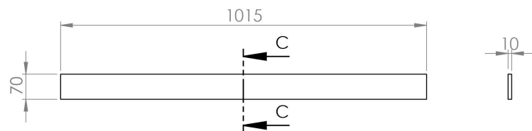
SECTION C-C
